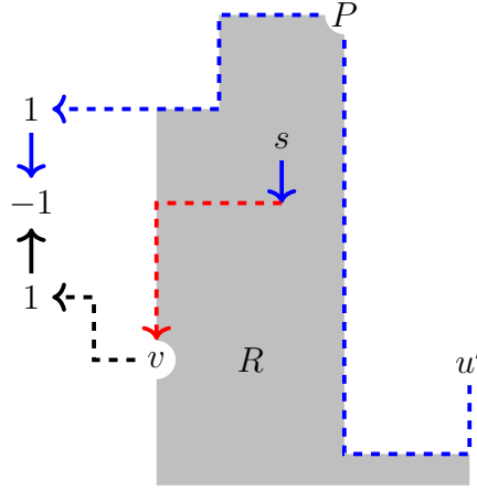
FIGURE 1. Proof of Claim 3.4 . The column containing the depicted \pm 1 's is strictly left of \text{col}(v) .
